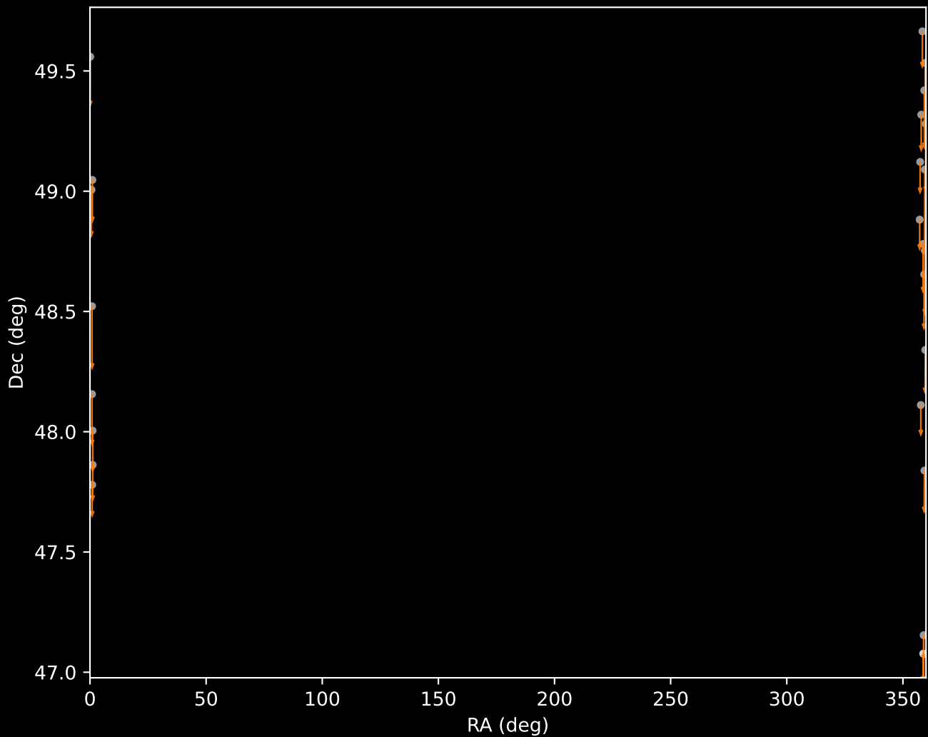
APOGEE DR17 Cluster 2 Proper Motion Vectors (n=25)
