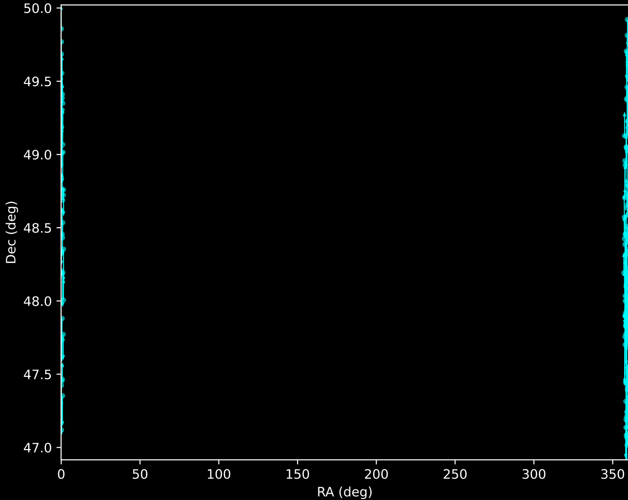
APOGEE DR17 Noise Stream Proper Motion Vectors (n=102)
