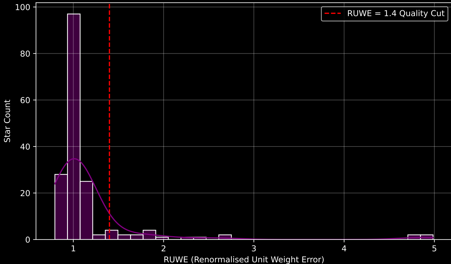
GAPOGEE DR17 Field [075+35] RUWE Distribution (n= 173)
