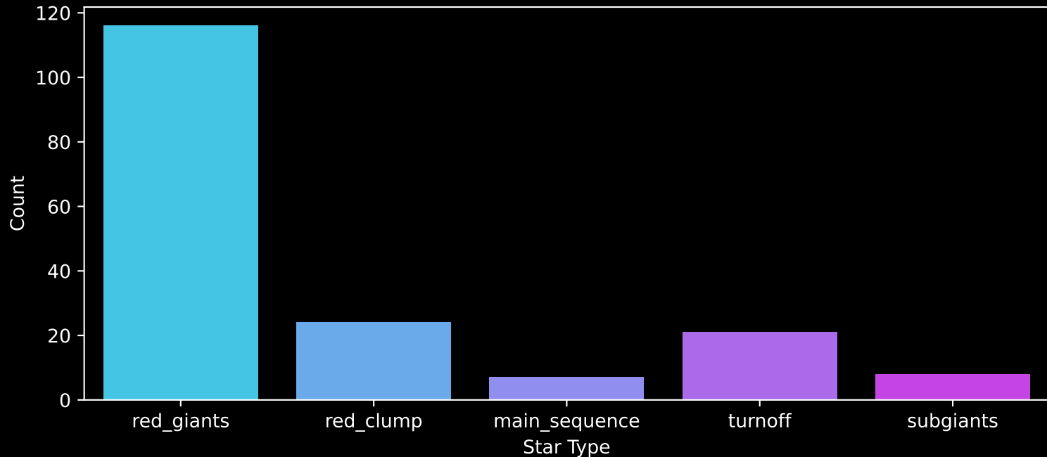
APOGEE DR17 Field: [075+35] Count plot of Star Type
