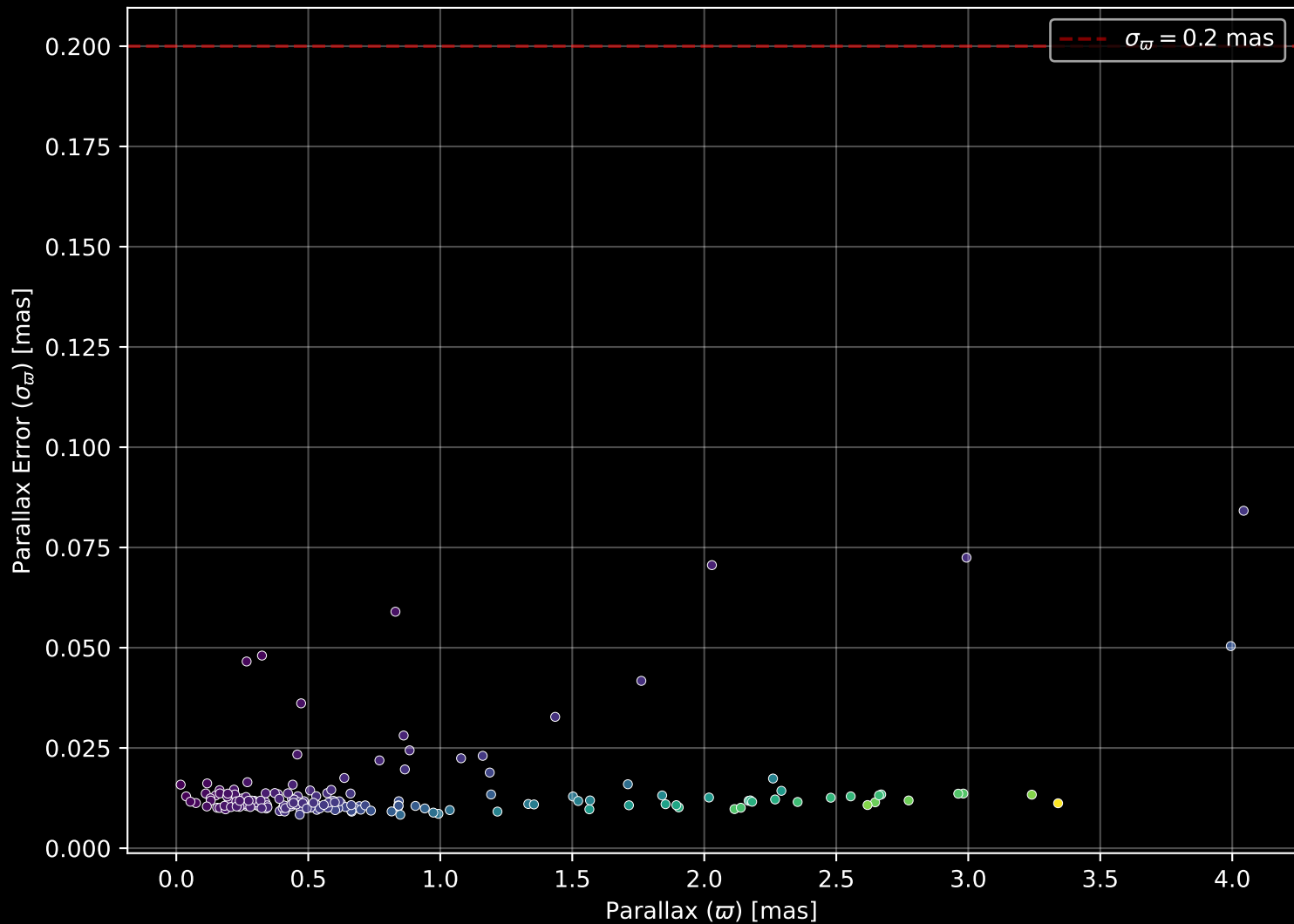
APOGEE DR17 Field: [075+35] Parallax Quality (n= 176)
