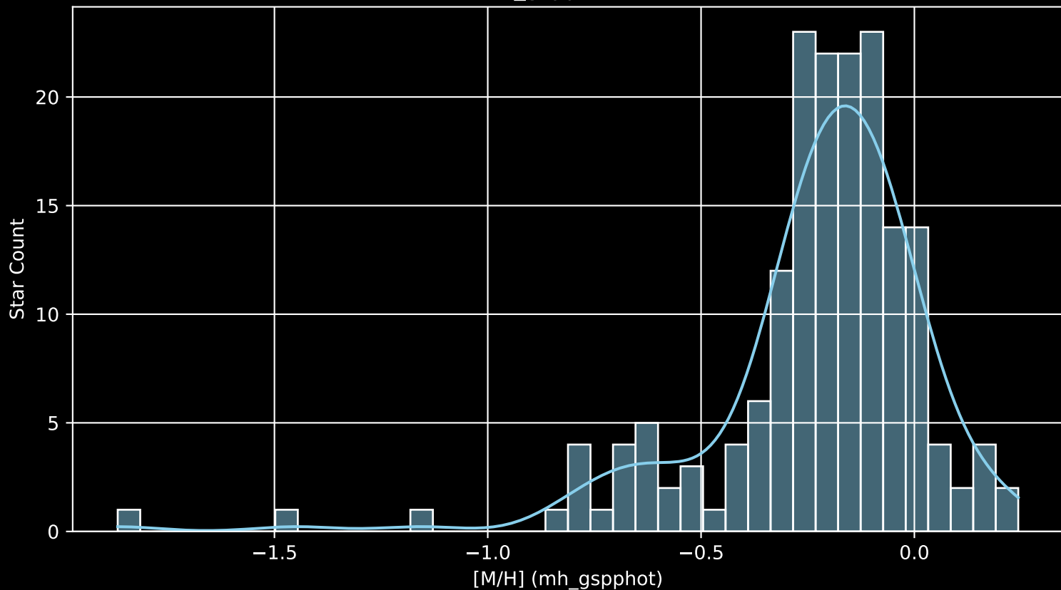
APOGEE DR17 Field: [075+35 [M/H] (mh_gspphot) (n= 176)
