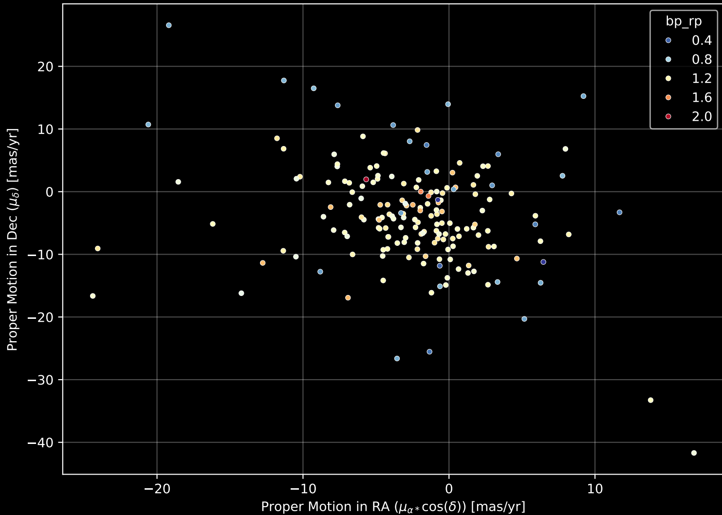
APOGEE DR17 Field: [075+35] Proper Motion Diagram (n= 176)
